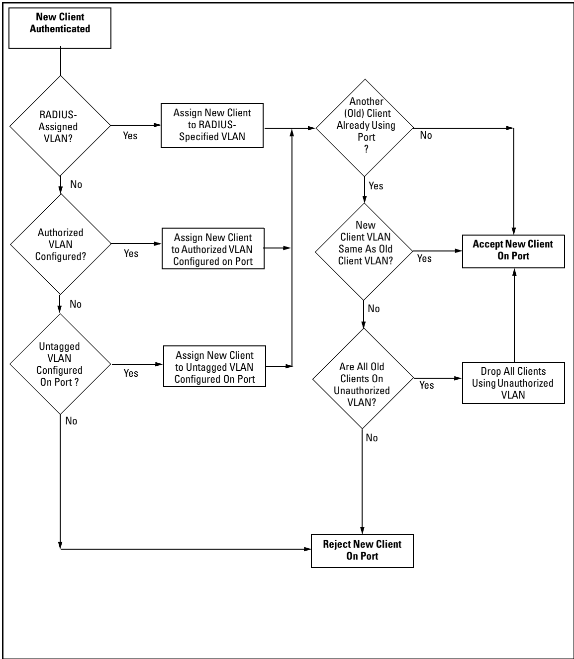
Figure 12-1. Priority of VLAN Assignment for an Authenticated Client
